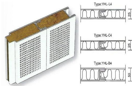
Type A Composite Rock Wool Perforated Sound Reduction Panel
